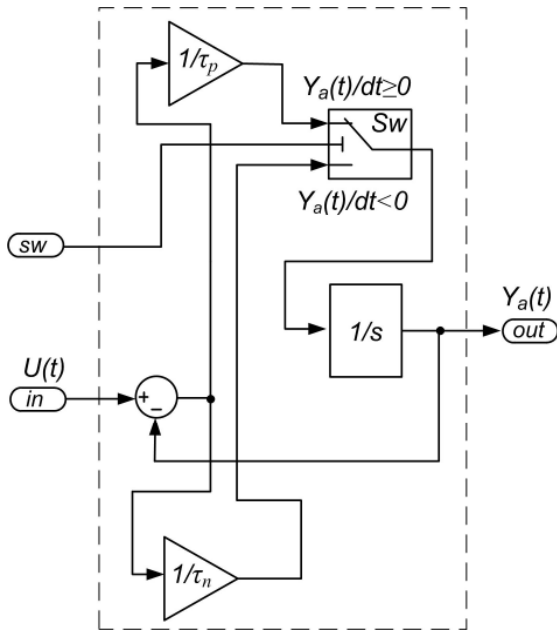
Fig. 3. The model of 1-st orders process with the asymmetric dynamics for the software Simulink
