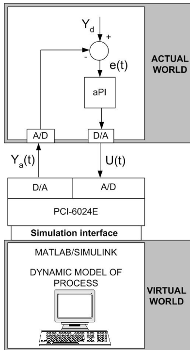
Fig. 2. The block diagram of the HIL simulation system for the investigation of aPI controller
