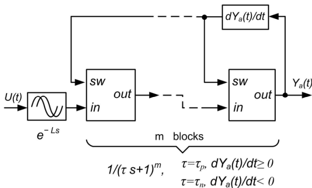
Fig. 4. The model of the m -order process with the asymmetric dynamics and response delay for the software Simulink
