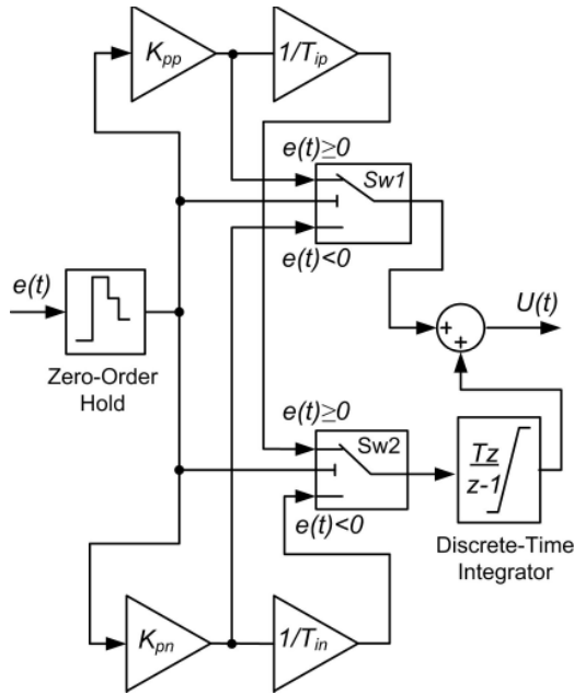
Fig. 1. The block diagram of digital aPI controller
