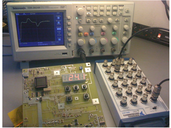
Fig. 5. The HIL simulation system for the investigation of aPI controller (the aPI controller is on the left, the connector block of multifunctional PC board PCI-6024E, which is connected to the PC with the installed Simulink software– on the right)
