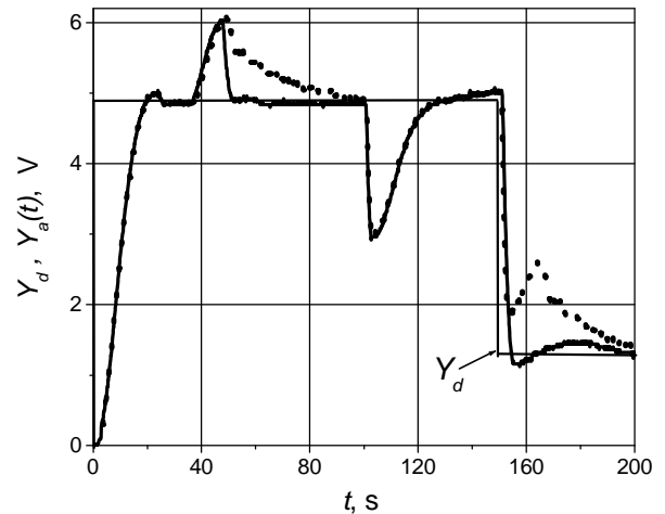
Fig. 6. Set point pulse and load disturbance response of the control system based on the aPI (solid line) and PI (dotted line) controllers. The PI controller parameters ( K_p=0.8 , T_i=10s ) are adjusted to dynamics of the process, which corresponds to the rise of controlled parameter. Parameters of aPI controller: K_{pp}=0.8 , K_{pn}=0.5 , T_{ip}=10s , T_{in}=2s
