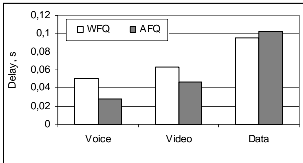
Fig. 7. Average delay time ( \rho = 0,50 to 0,70 )
