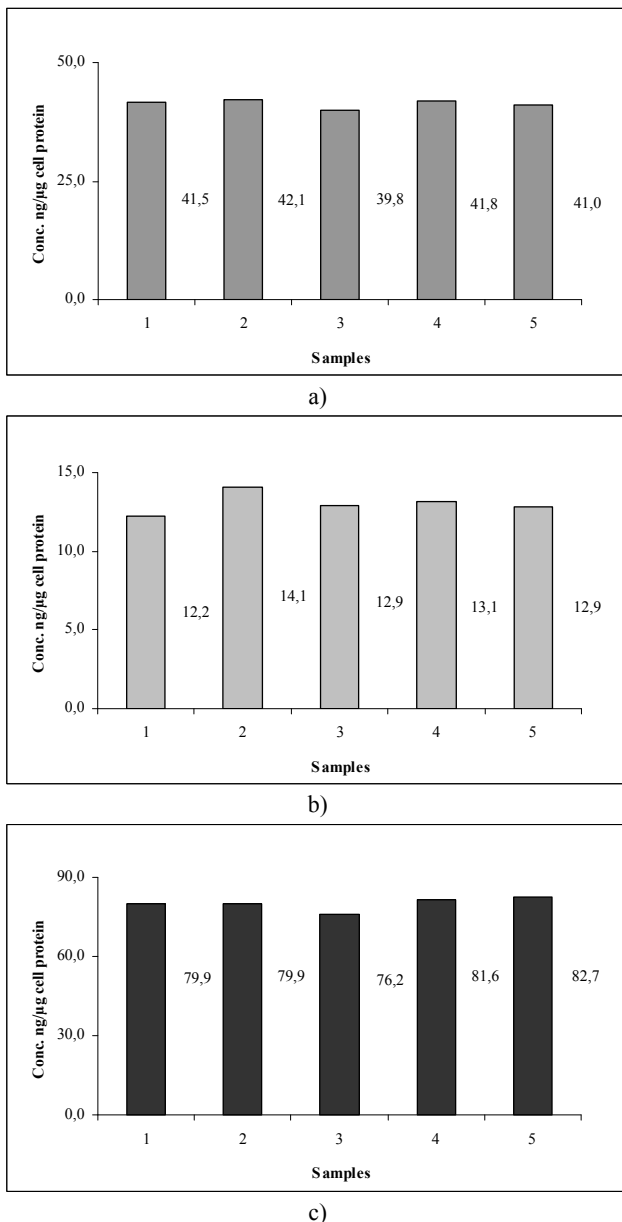
Fig. 2. Concentration of: a – oleic acid in human hepatoma G2 cells; b – stearic acid in human hepatoma G2 cells; c – palmitic acid in human hepatoma G2 cells
