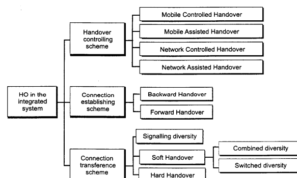
Fig. 1. Handover taxonomy for satellite/terrestrial network architecture
