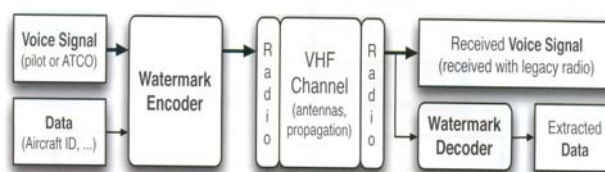
Fig. 2. Watermarking system for the aeronautic radio
