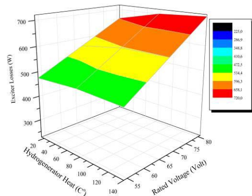
Fig. 2. HG's heat and the rated voltages variation with the exciter loss
