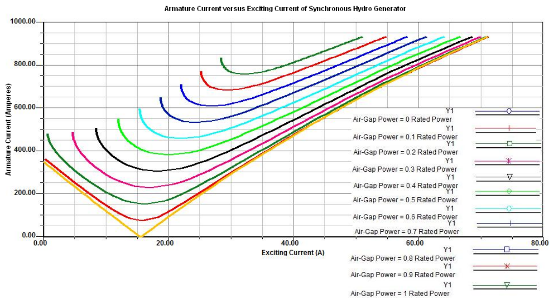
Fig. 5. V Curves of the HG (Armature current versus exciting current)
