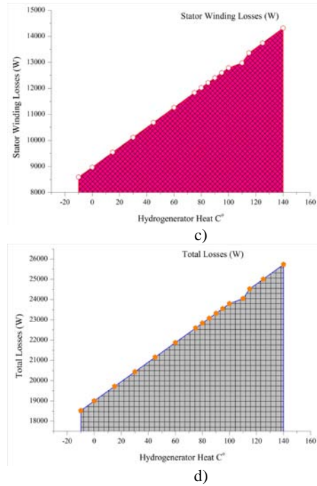
Fig. 4. Power losses variation with HG's heat (Watts versus C°): a – field winding losses; b – iron losses; c – stator winding losses; d – total losses
