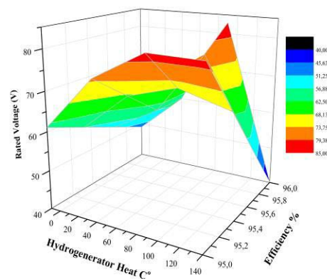
Fig. 3. HG's heat and the rated voltages variation with the efficiency
