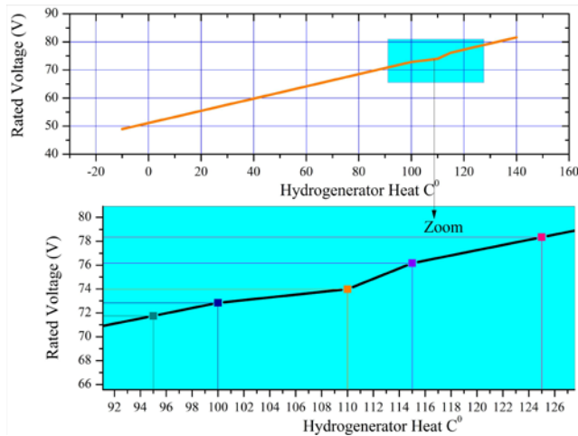
Fig. 1. Exciter voltage variation with hydrogenerator heat
