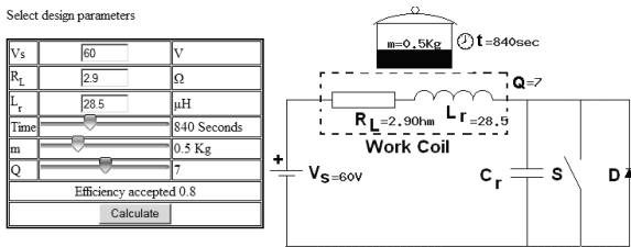
Fig. 2. Index page of the SSRI desing web site
