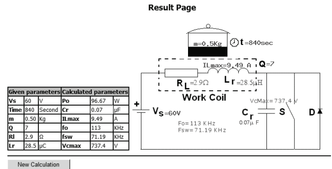
Fig. 4. Result page of the SSRI design tool
