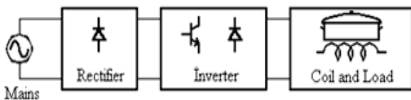
Fig. 1. Induction cooking block diagram
