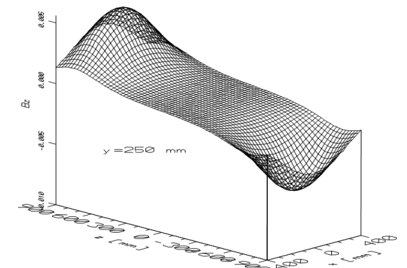
Fig. 3c. Component Bz for rectangular loop (dimensions 1500 x 500 mm), 250 above the loop
