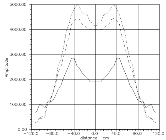
Fig. 14. Pulse amplitude as a function of metal carriage offset \Delta x
