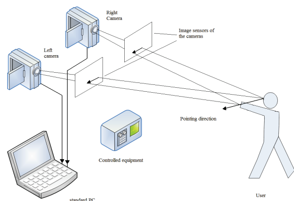
Fig. 1. The layout of interaction components for the system of determining user's pointing direction
