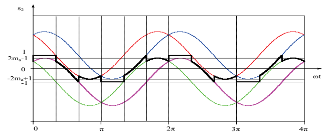
Fig. 1. The modulator signal DPWM-S2
