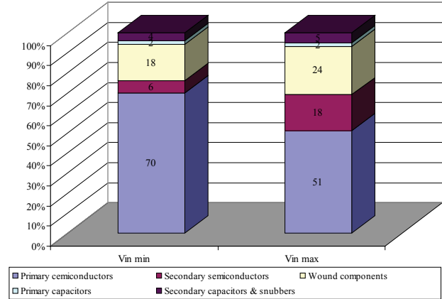
Fig. 6. Loss distribution in different operating modes
