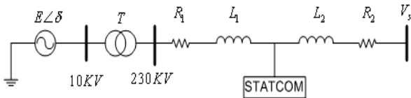
Fig. 3. Schematic diagram of simulation system
