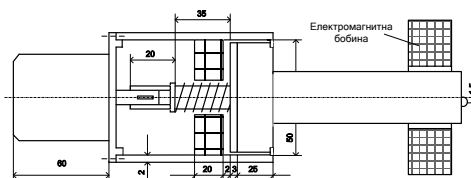
Fig. 9. Modified mechanical device for acupressure simultaneously with application of low frequency magnetic filed
