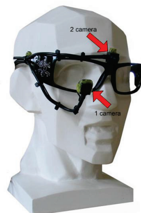
Fig. 10. The head rotation compensation device
