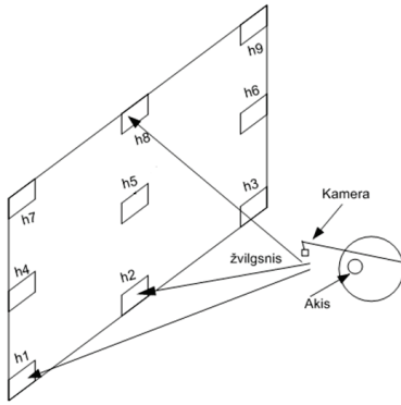
Fig. 4. Calibration points displayed on the monitor screen
