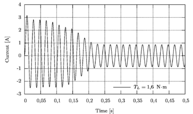
Fig. 5. Simulation results of current transients at no load and with rated load
