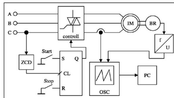
Fig. 1. Block diagram of experimental equipment
