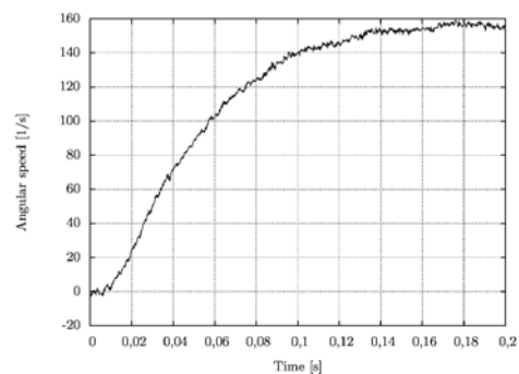
Fig. 6. Speed transients at starting (experimental)
