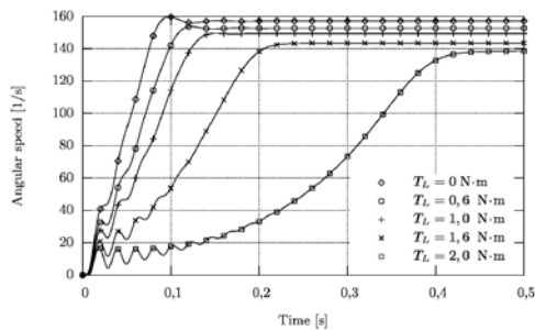
Fig. 7. Simulation results of speed transients
