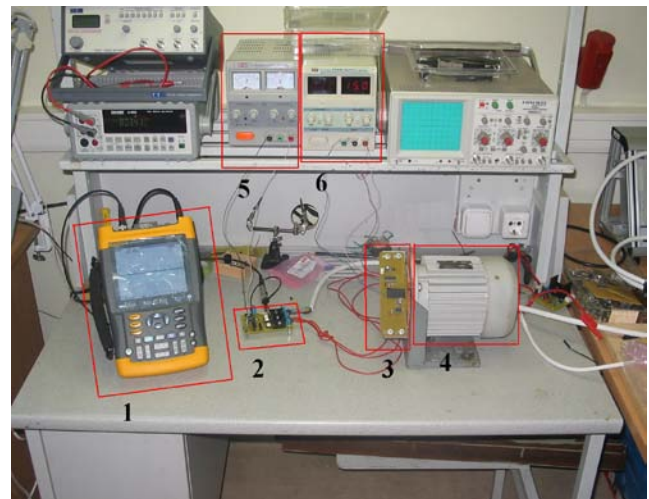
Fig. 3. Experimental equipment: 1 – oscilloscope; 2 – symistor relay; 3 – digital tachometer; 4 – induction motor; 5 – supply source of control part; 6 – supply source of digital tachometer
