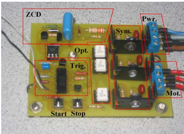
Fig. 2. Control part of experimental equipment
