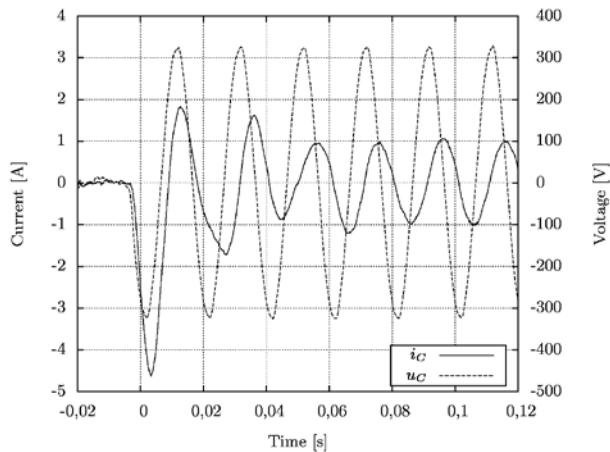
Fig. 4. Experimental transients of stator C phase voltage and current
