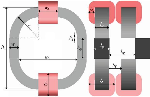
Fig. 2. Simulator model of the actuator
