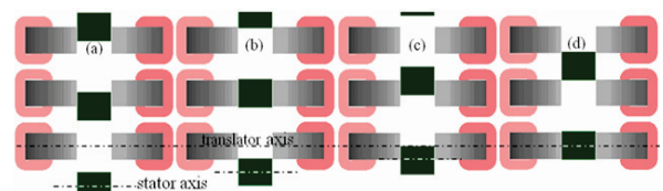
Fig. 4. Stator and translator positions a – fully unaligned; b – overlap; c – mid-aligned; d – fully aligned
