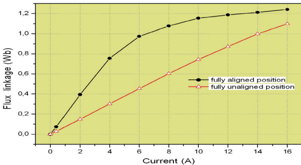
Fig. 7. Flux linkage profile of the actuator
