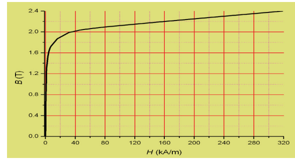
Fig. 3. The B-H curve of rotor and stator core material
