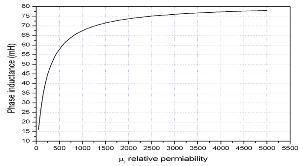
Fig. 8. The impact of relative permeability on inductance
