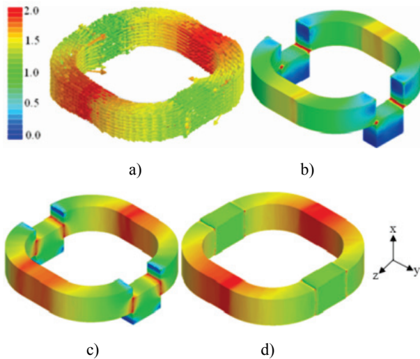
Fig. 11. a – Vectoral distribution of B in fully aligned position, amplitude distribution of B ; b – overlap; c – mid-aligned; d – fully aligned positions
