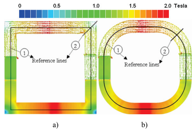
Fig. 9. Reference lines and magnetic flux distribution a- quadrangular core b- circular core
