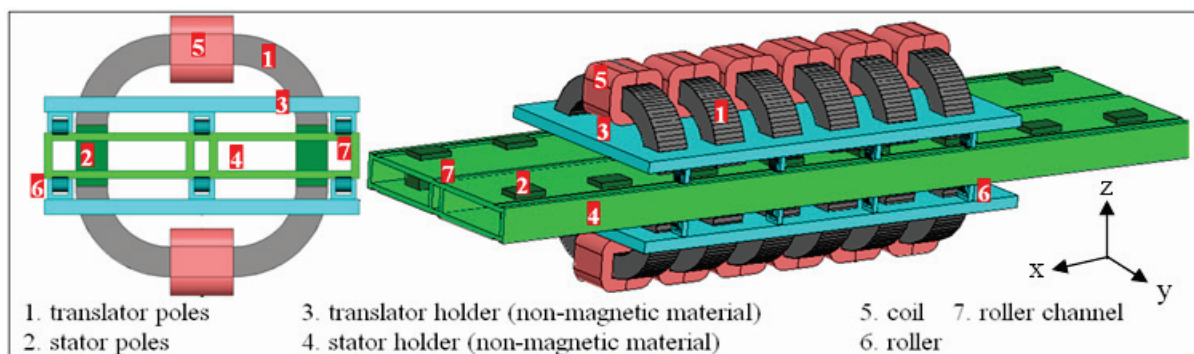
Fig. 1. Simulated model of the linear actuator
