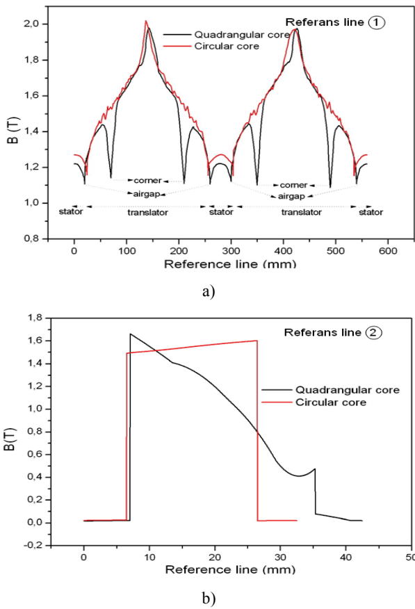
Fig. 10. Magnetic flux density in the reference lines: a – 1st reference line; b – 2nd reference line
