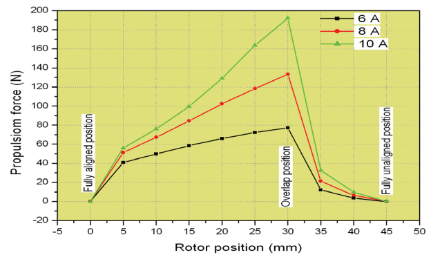
Fig. 12. Force profile of the actuator
