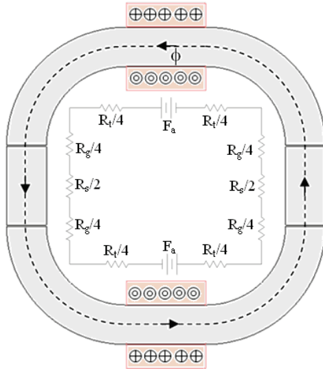
Fig. 5. Actuator core flux path and magnetic circuit
