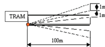
Fig. 3. LIDARs beam geometry
