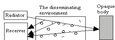
Fig. 1. LIDARs working principle
