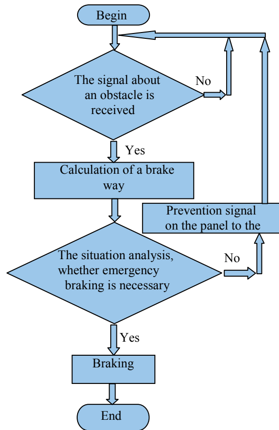
Fig. 2. The block diagram of simple trams braking systems managing algorithm
