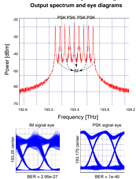
Fig. 6. Mixed WDM system output spectrum after 40 km fiber length. The worst received eye diagrams presented for each modulation technique, 75 GHz channel interval and DSF fiber is installed
