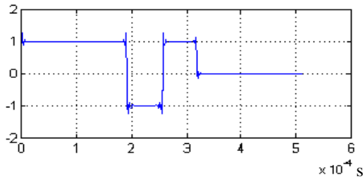
Fig. 2. Sensor output after FDFIB compensation
