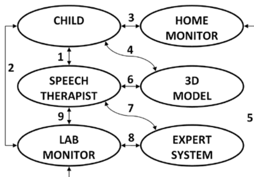
Fig. 1. Architecture of the Logomon system
