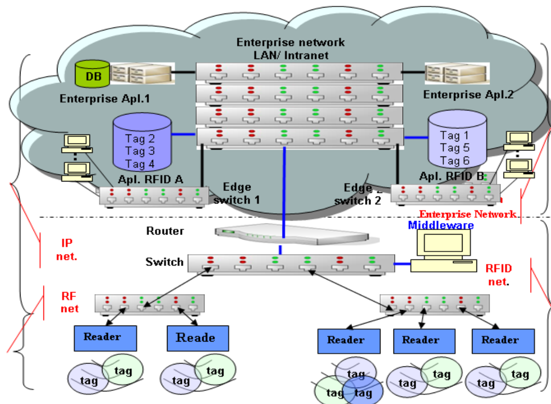
Fig. 5. Dedicated network
