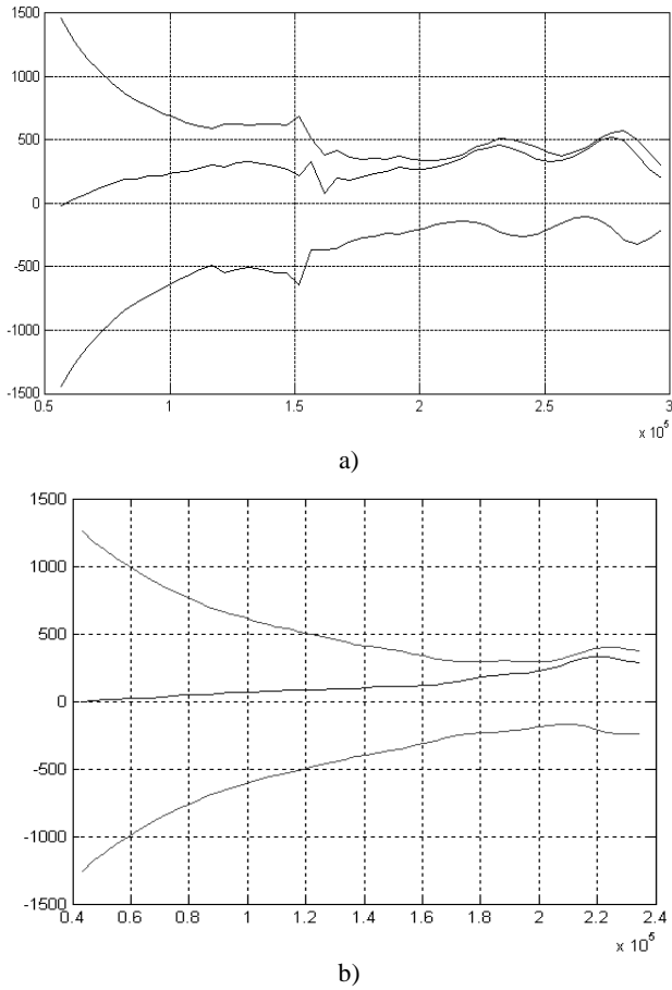
Fig. 5. PZT (S3) impedance of simultaneous multi-frequency method (a) measured by using of 5 kHz frequency grid, in (b) the used frequencies has been shifted by 2 kHz from the 5 kHz grid
