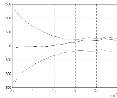
Fig. 4. PZT (S3) impedance for frequency scanning method
