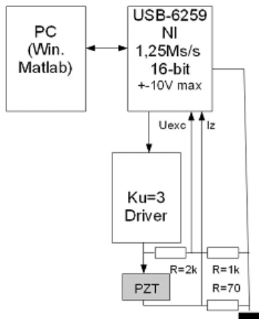
Fig. 1. Measurement setup (block diagram)
