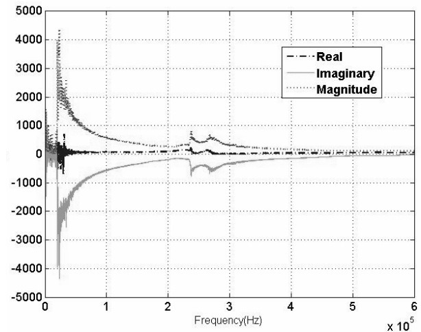
Fig. 7. PZT (S3) impedance obtained by the aid of a chirp (80ms) signal
