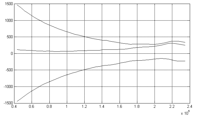
Fig. 6. PZT (S3) impedance obtained by the modified simultaneous multi-frequency method, by using 4x FFT and 1/4 shift of frequency values
