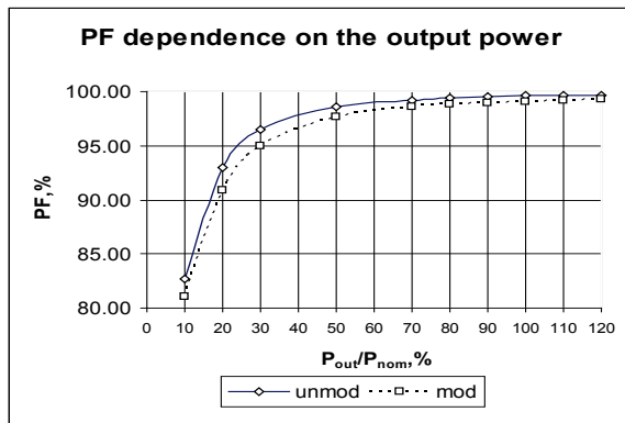
Fig. 4. The dependence of PF on the output power
