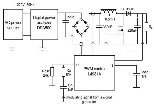
Fig. 3. Simplified schematic diagram of the experimental setup
