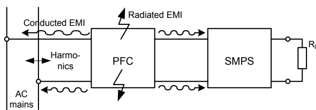
Fig. 1. Utility interface with typical power supply for DC load
