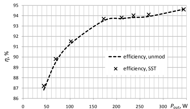
Fig. 6. Efficiency \eta vs. P_{out} ( f_{sw} = 100\text{kHz} ; \Delta f_{sw} = 30\text{kHz} ; f_m = 2.5\text{kHz} )
