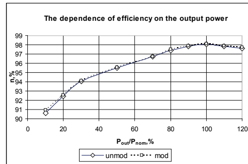
Fig. 5. The dependence of efficiency of PFC on the output power
