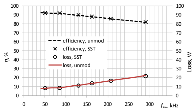
Fig. 7. Efficiency and loss vs. switching frequency ( \Delta f_{sw} = 30\text{kHz} ; f_m = 2.5\text{kHz} )
