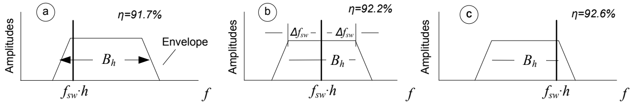
Fig. 2. Transformation of the harmonic h of the switching frequency f_{sw} into the appropriate band B_h in a consequence of FM of f_{sw} : b – for symmetrical FM; a, c – for asymmetrical ones
