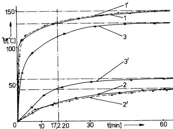
Fig. 2. The heating transitory evolution
