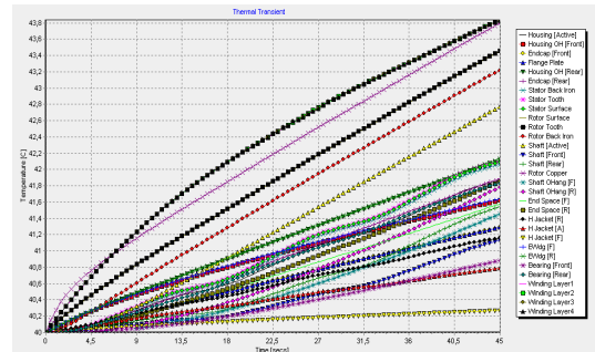
Fig. 7. Thermal values in the different parts of the motor
