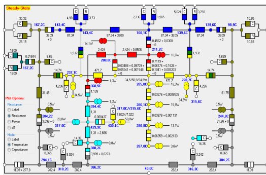
Fig. 9. Steady-state scheme for Teflon material
