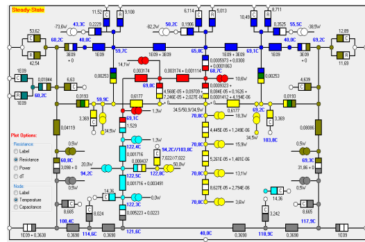
Fig. 6. Steady-state scheme for aluminum
