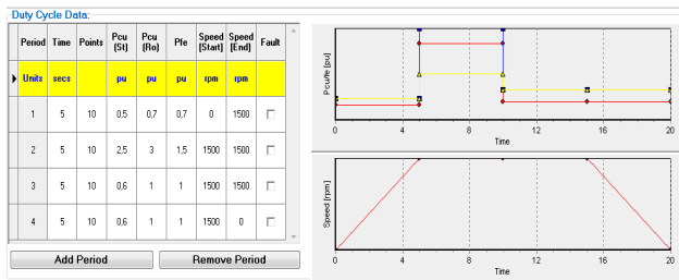
Fig. 5. Speed, acceleration and load values of the motor
