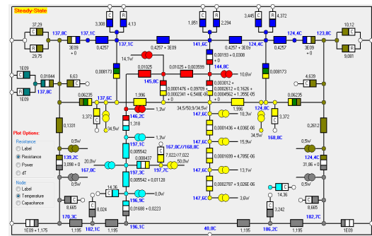
Fig. 8. Steady-state scheme for cast-iron
