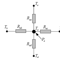
Fig. 1. The basic thermal network constituting the system
