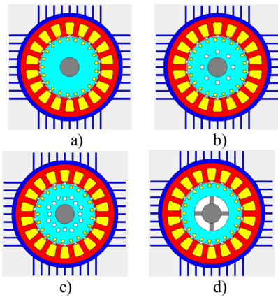
Fig. 4. Different rotor types and different short circuit bars
