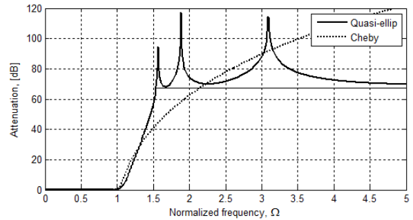
Fig. 5. Comparative curves of the attenuation for quasi-elliptic and Chebyshev prototypes
