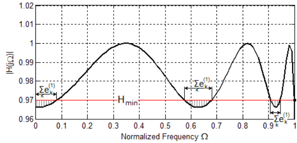
Fig. 2. Forming AFR error in pass band
