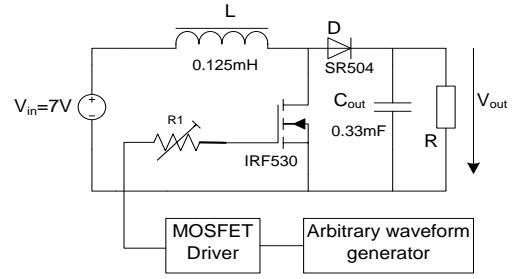
Fig. 9. Simplified schematic diagram of the experimental setup
