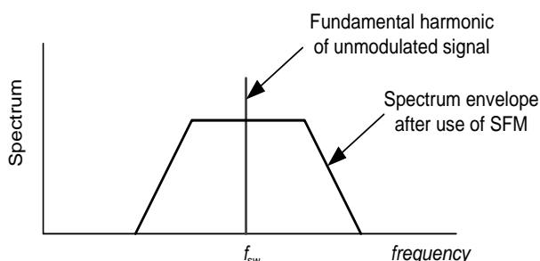
Fig. 1. Simplified spectral structure of a switching signal before and after using SFM
