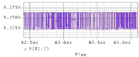
Fig. 7. Simulated output voltage ripples of the SFM boost converter in CCM ( L=125\mu\text{H} ; C_{out}=330\mu\text{F} ; V_{in}=7\text{V} ; R_{out}=12\Omega ; D=0.3 ; modulation parameters: sinusoidal modulation; f_{swc}=100\text{kHz} ; f_m=1\text{kHz} ; \Delta f_{sw}=30\text{kHz} ; parasitic parameters: t_d=0\text{ns} ; r_{loss}=0.6\Omega ; r_c=0.035\Omega )
