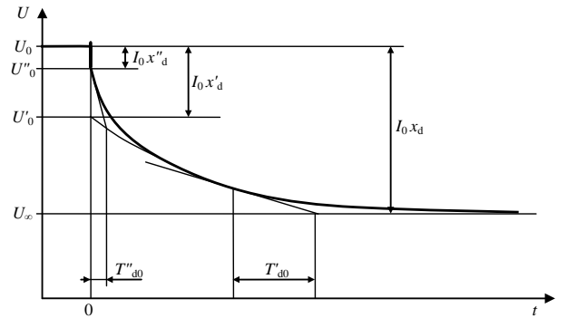
Fig. 2. The variation in voltage when the generator loaded with capacitive reactive load was switched off
