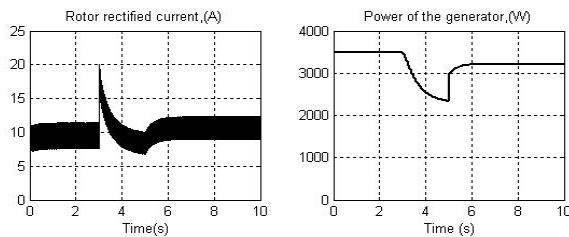
Fig. 5. Curves of the WT's power conversion system parameters at the jump of generator's load reference signal U_v from 6 to 7 V after 3 s, drop of the wind speed v_w from 12 to 9 m/s at t = 5 s and switching on the boiler feeding at t = 7 s
