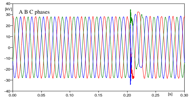
Fig. 7. Overvoltages at junction of overhead line and cable for scenario (d)
