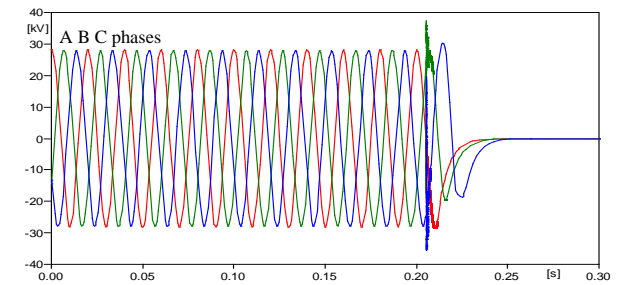
Fig. 8. Overvoltages at 2 km (almost same at 4 km) away from surge arrester (near fuse) for scenario (d)
