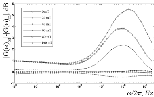
Fig. 2. Diagram of differences between AFCh of ITF images of seed impacted and unimpacted by magnetic field
