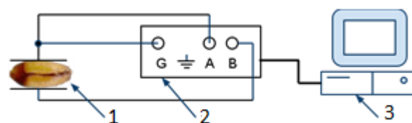
Fig. 1. Structural diagram of research ITF frequency characteristics: 1 – grain and electrodes; 2 – A/D converter; 3 – PC, G – output of oscillator; A,B – inputs of A/D converter
