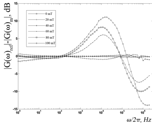
Fig. 3. Diagram of difference between PFCh images of seed impacted and unimpacted by magnetic field
