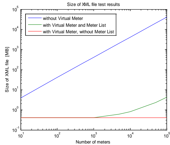
Fig. 6. Size of exported file
