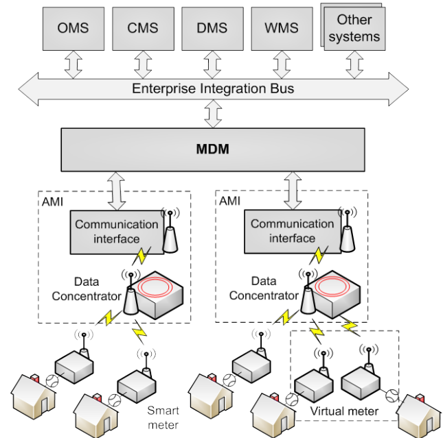
Fig. 1. Open Smart Metering architecture
