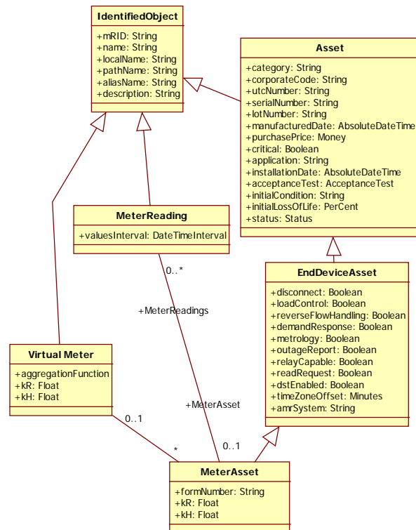
Fig. 2. CIM model with Virtual Meter
