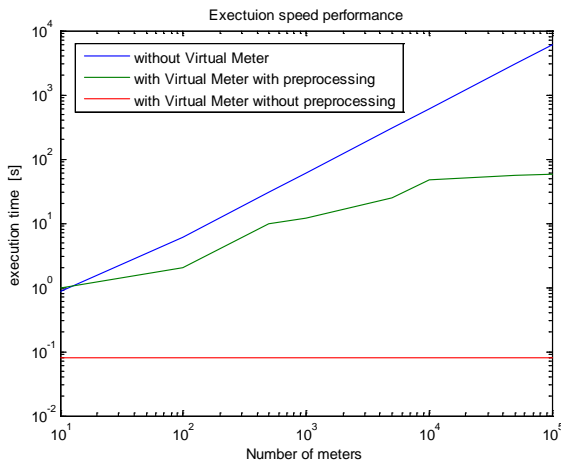
Fig. 5. Speed or execution performance test
