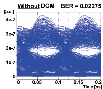
Fig. 9. Output eye diagram for the second channel of 10 Gbit/s 4 channel WDM system without dispersion compensation
