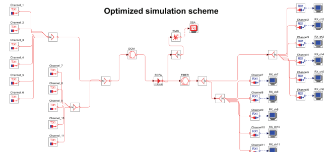
Fig. 4. Simulation model of optimized bidirectional DWDM solution
