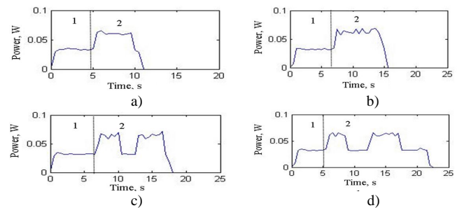
Fig. 4. Data transfer waveforms a – ideal mode; b, c, d – real environment.
