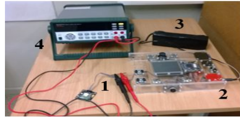
Fig. 3. Implementation view 1 -CM, 2 – CPM, 3 – PS, 4 – multimeter.
