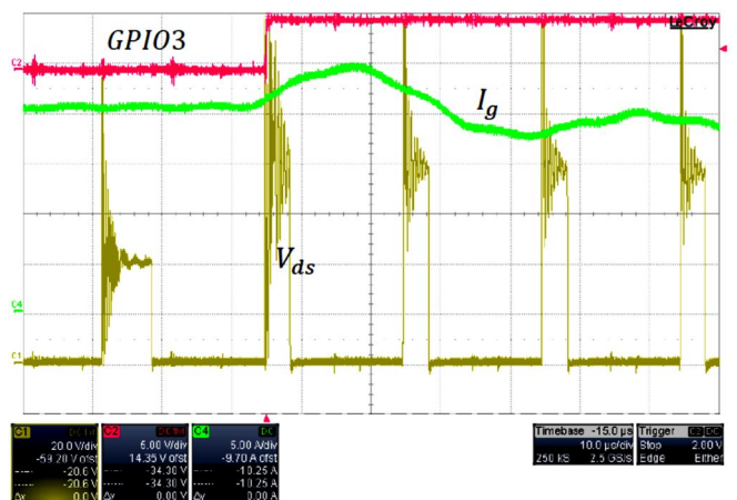
Fig. 23. Detailed zoomed waveforms of the transition Time scale: 10 µs/div). Source output current I_g (green, 5 A/div), primary MOSFET drain to source voltage (brown, 20 V/div) and short circuit control signal GPIO3 (red, 5 V/div).
