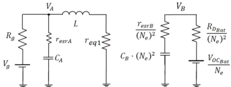
Fig. 12. PPIBC simplified equivalent circuit during the inductor charge.
