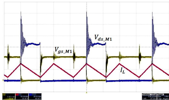
Fig. 18. Converter operating waveform during normal operation mode. M1 gate signal (brown, 5 V/div), M1 drain to source voltage signal (blue, 20 V/div) time scale 5 µs/div.
