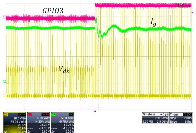
Fig. 22. Transition between operating modes with pre-calculated steady-state duty cycle. Time scale: 200 µs/div. Source output current I_g (green, 5 A/div), primary MOSFET drain to source voltage (brown, 20 V/div) and short circuit control signal GPIO3 (red, 5 V/div).
