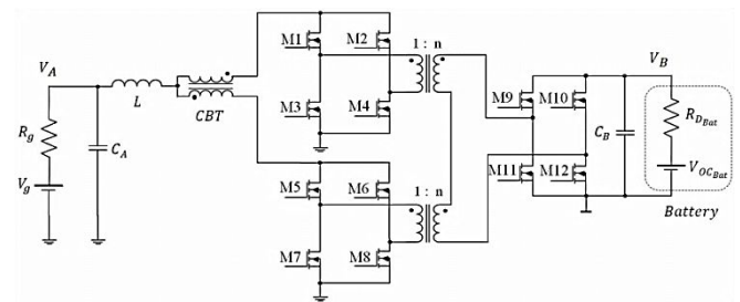
Fig. 1. Primary parallel isolated boost converter schematic.
