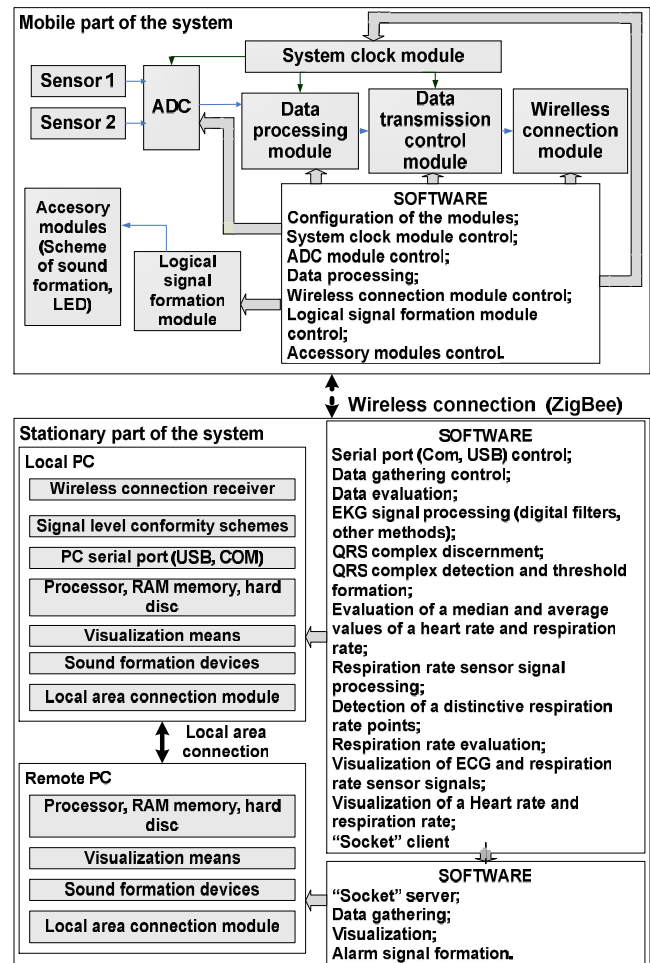
Fig. 2. Structure of the physiological parameter monitoring system.
