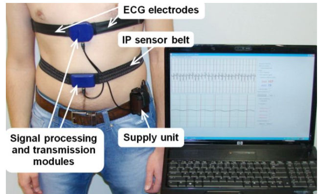
Fig. 1. View of the physiological parameter monitoring system.
