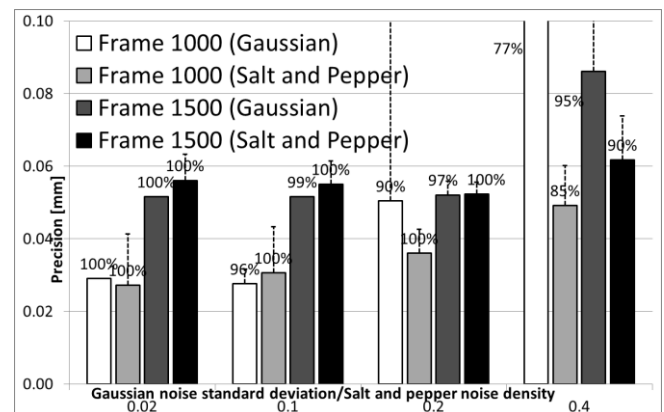
Fig. 5. Optimal cropping frames for both Gaussian and salt and pepper noises.
