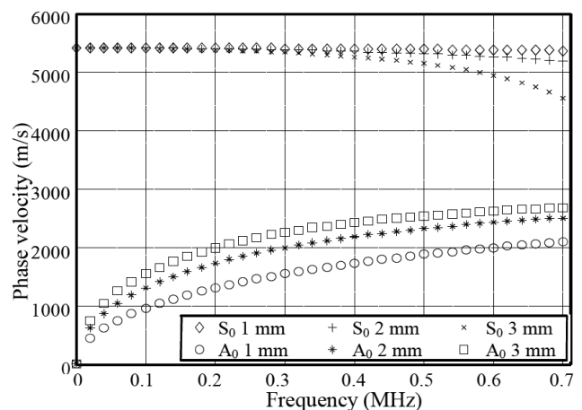
Fig. 1. The theoretical phase velocity c_{ph} dispersion curves of the asymmetric A_0 and symmetric S_0 Lamb waves modes propagating in 1\div 3 mm thickness aluminium alloy plates.
