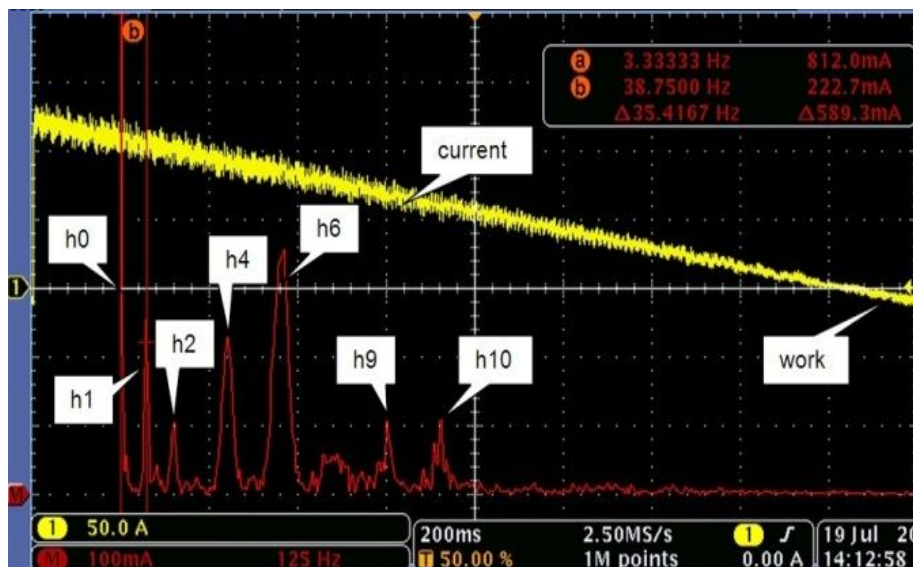
Fig. 9. Current waveform during the braking process with FFT analysis results [7].
