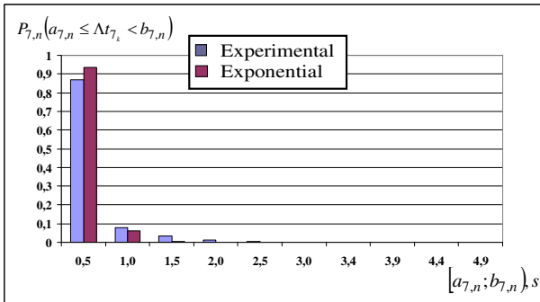
Fig. 10. Probability histogram of any type signalling messages inter-arrival time at SIP PS.
