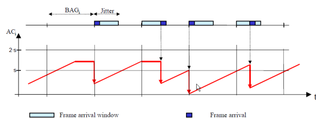
Fig. 1. Traffic without jitter.
