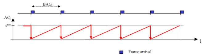
Fig. 2. Traffic with jitter = BAG/2.
