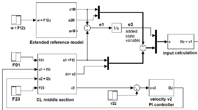
Fig. 4 Block diagram of CL tension control.
