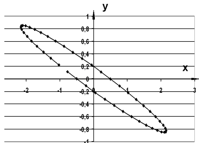
Fig. 3. A trajectory of the magnetic field vector for the five-phase winding of the third harmonic
