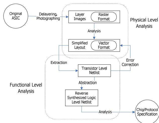
Fig. 1. Reverse engineering procedure
