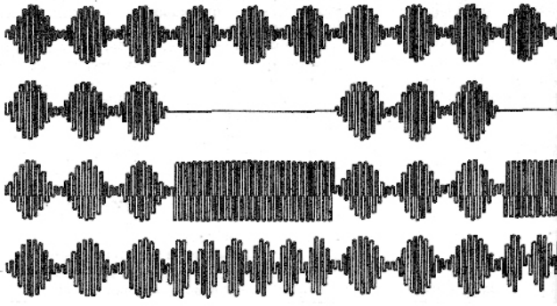
Fig. 2. Output signals of apparatus AMPLIPULS
