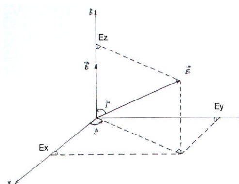
Fig. 1. Disposition of vectors \vec{E}(x, y, z, t) and \vec{B}(x, y, z, t)
