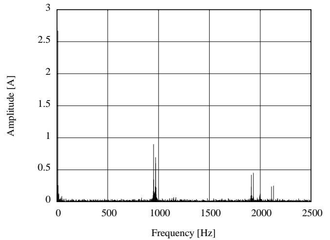
Fig. 5. Motor current spectrum at f_p = 10 Hz
