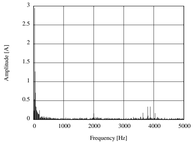
Fig. 6. Motor current spectrum at f_p = 40 Hz
