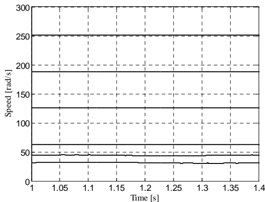
Fig. 2. Experimental results of motor steady-state speed at no-load at different f_p given in Table 2
