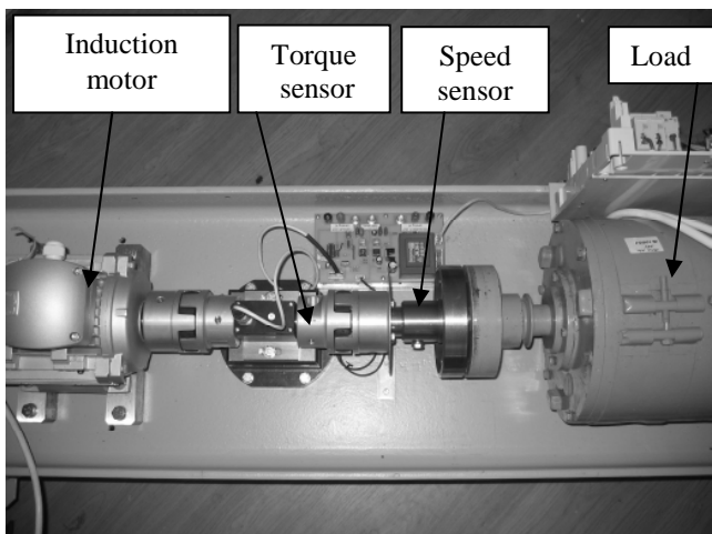
Fig. 4. The laboratory setup for experimental investigation
