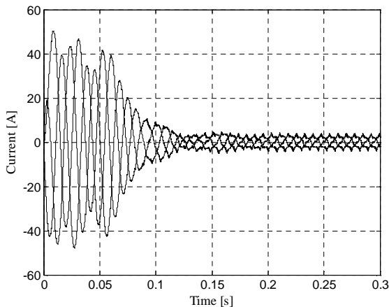
Fig. 3. Starting transients of motor current at no load at f_c = 4320 Hz, f_p = 45 Hz
