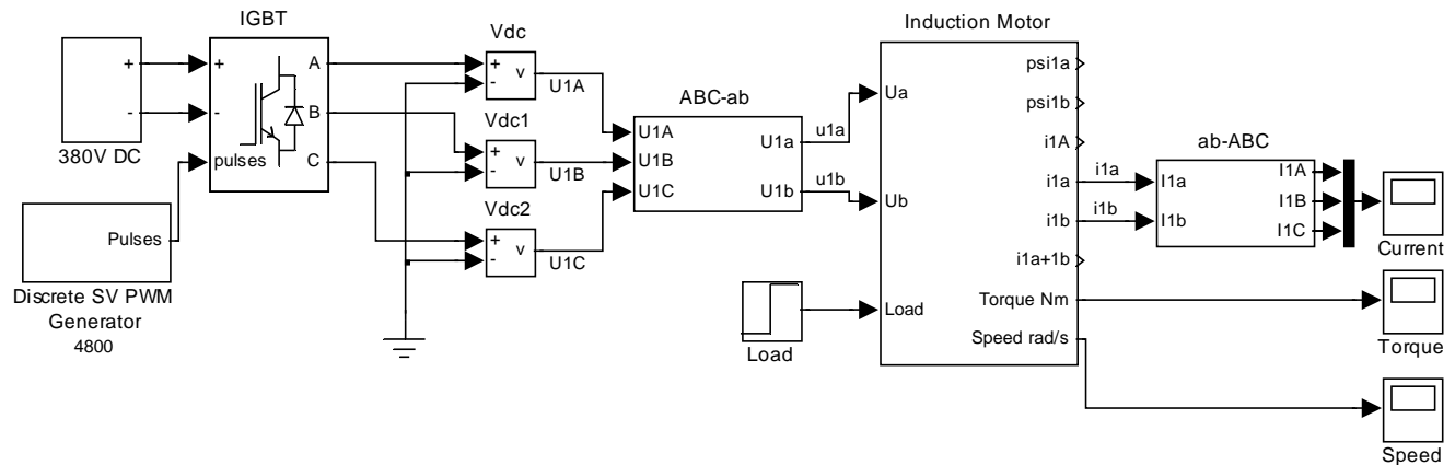
Fig. 1. The Simulink model of the induction motor supplied by the frequency converter
