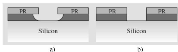
Fig. 1. Etch through a photoresist (PR) mask: a – isotropic etching is independent of the plan the crystal; b – anisotropic etching is dependent on the plane of orientation [4]
