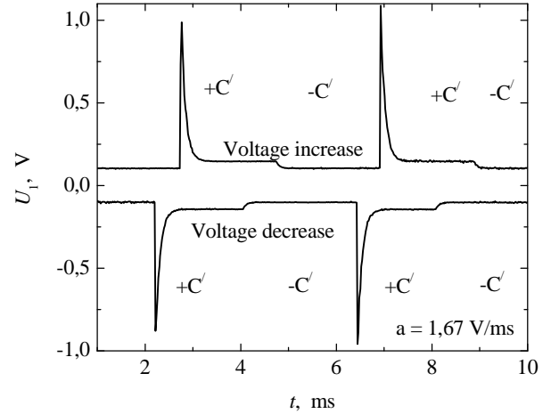
Fig. 2. Experimentally measured regularities of output voltage changes due to jump increase (+ C' ) or jump decrease -C' of the measured capacitance
