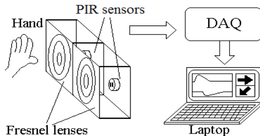
Fig. 7. Experimental setup
