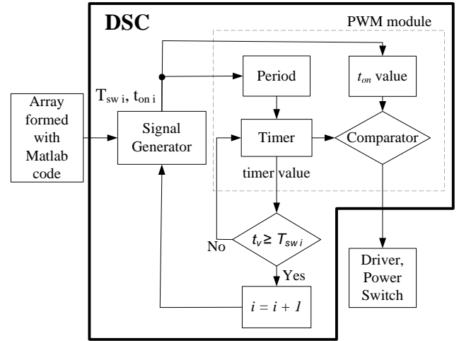
Fig. 3. PWM signal forming algorithm implemented in DSC
