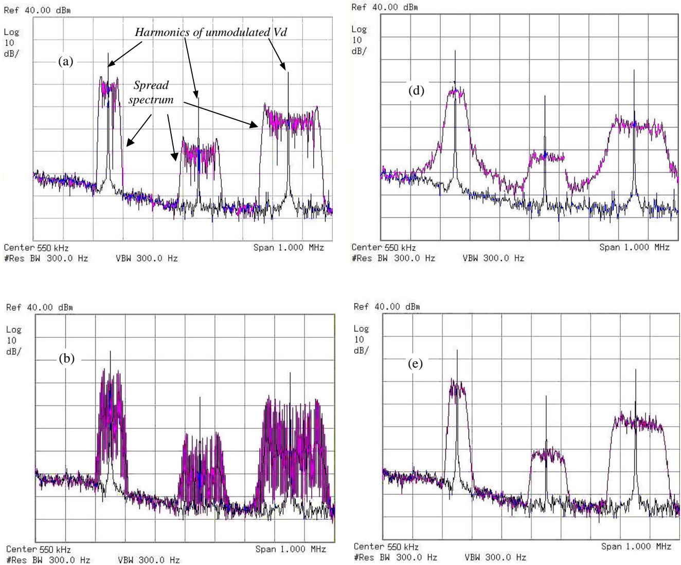
Fig. 6. Experimental power spectra of V_d for FM techniques examined with \Delta f_{sw} = 30\text{ kHz} . (a) SSFMT1. (b) SSFMT2. (c) PRSFMT2. (d) PRSFMT1. (e) PCSFMT. Comparison of Fig.6(a,b,e) with Fig.6(c,d) reveals that for pseudo-random SFMT EMI is spread along the whole frequency spectrum more evenly, while in the case of sinusoidal and pseudo-chaotic SFMT there are no distinct additional spectrum components between adjacent bands
