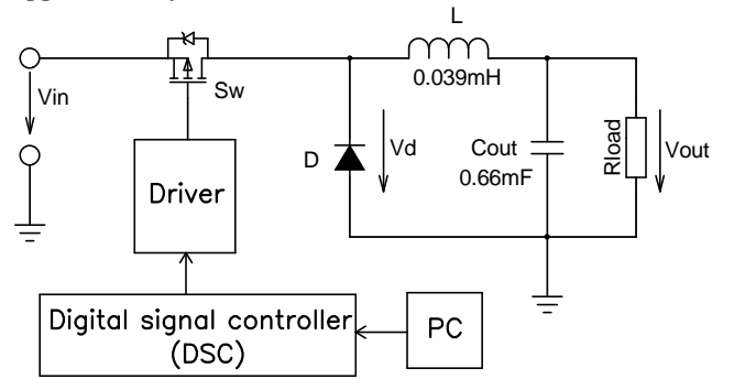
Fig. 2. Simplified schematic diagram of tested setup
