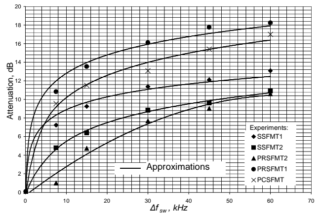
Fig. 4. Attenuation trends of the first harmonic of V_d with increasing \Delta f_{sw} , based on measured values
