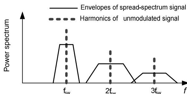
Fig.1. Comparison of switching signal as unmodulated and a spread-spectrum one
