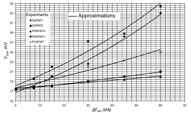
Fig. 5. Measured output voltage V_{p-p} versus \Delta f_{sw}
