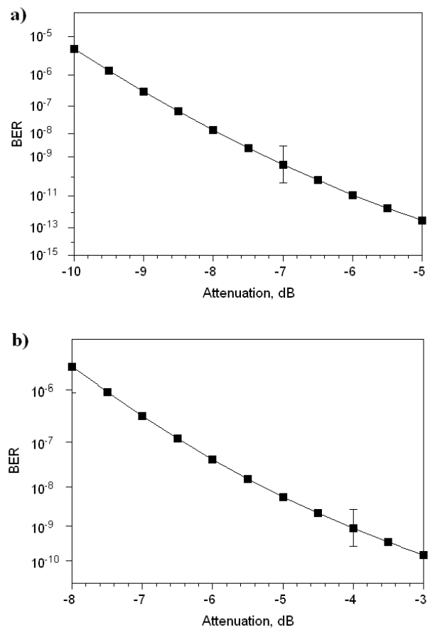
Fig. 4. BER dependence of inserted attenuation for a) 622 Mbit/s; b) 1 Gbit/s
